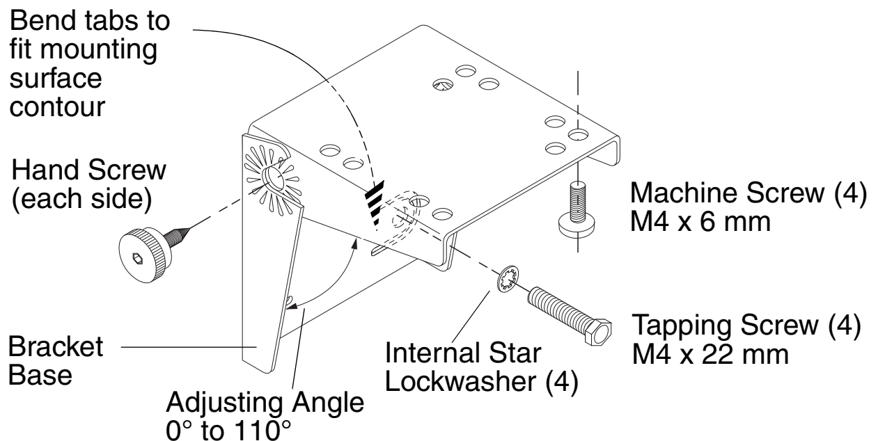
Figure 1. Adjustable Angle Bracket
